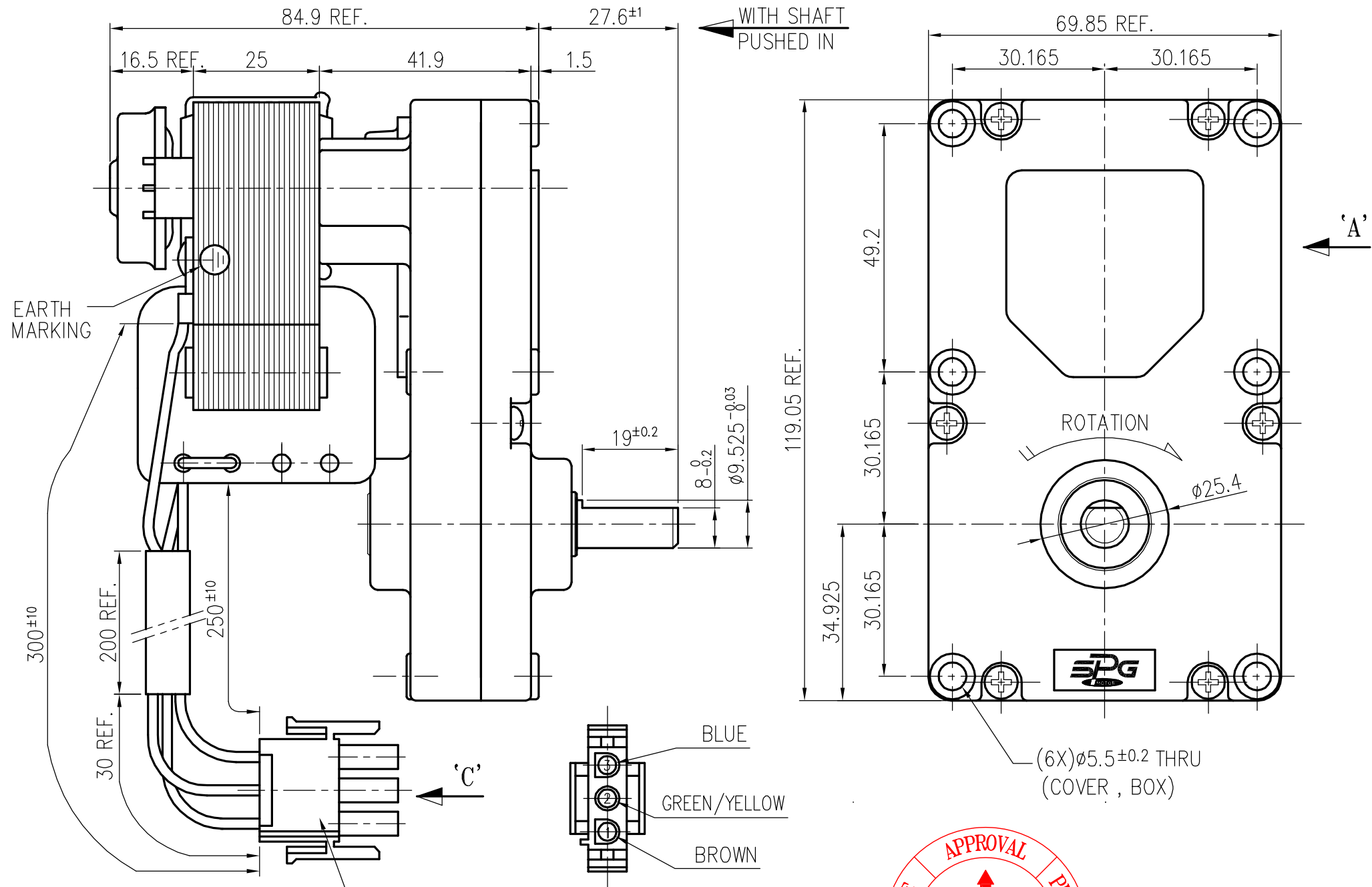
VIEW 'C'
